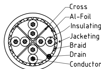
Wire Details
